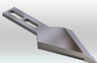
LÂMINA CENTRAL 58X150X4MM Cód. IMESC: 112121 Ref. Original: [REDACTED]
