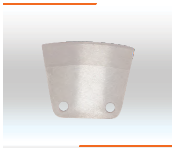
NAVALHA DORSO 36,40x43,50x2,50mm Cód. IMESC: 446227 Ref. Original: 0990.IDC1.015.00
