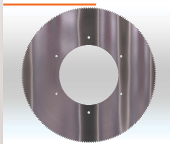
SERRA CIRCULAR DENTADO Ø450x200x1,20mm Cód. IMESC: 350324 Ref. Original: DISK450RBPK12Z282
